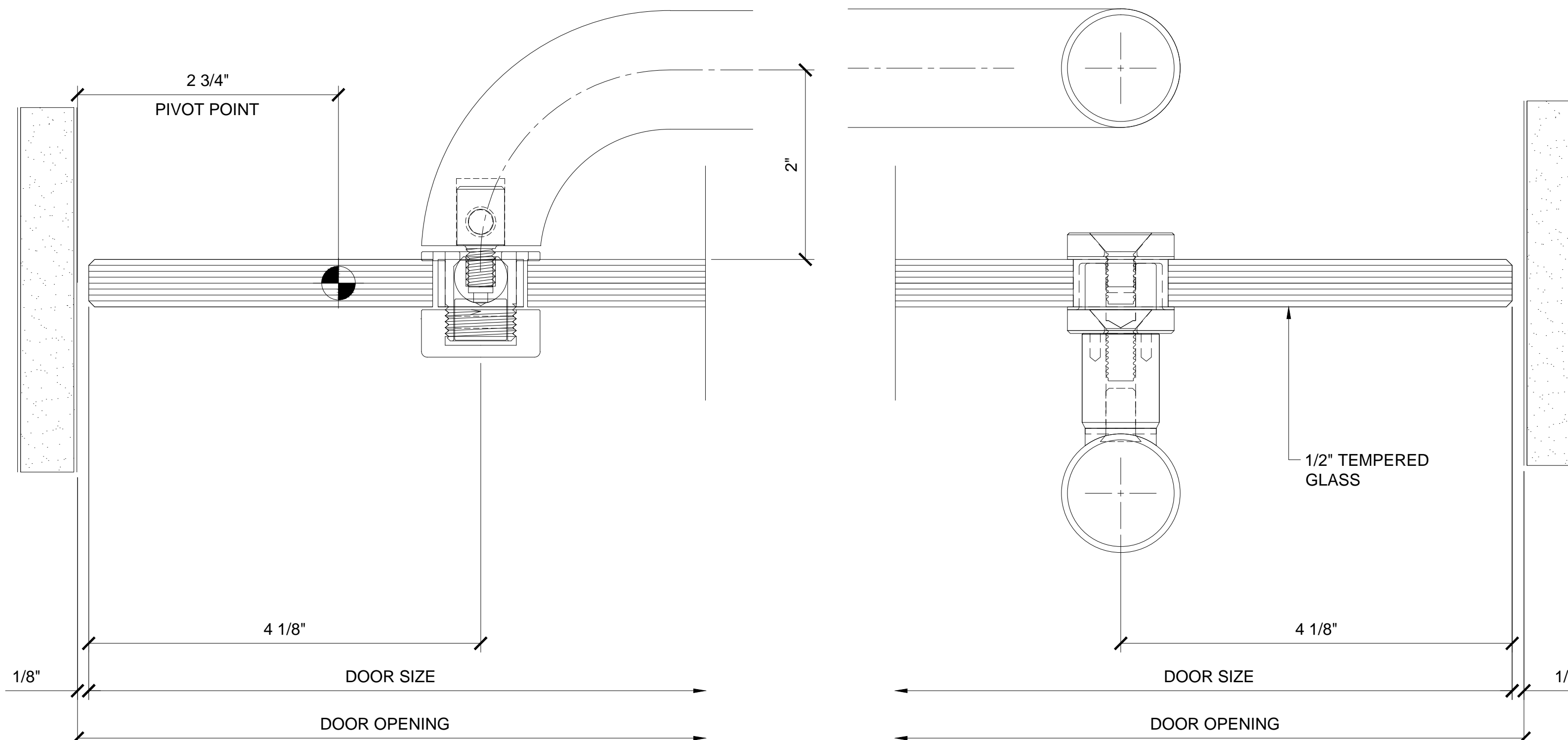
5 JAMB DETAIL AT PANIC HANDLE HINGE SIDE PATCH STYLE ALL GLASS DOOR W/ PA100F
