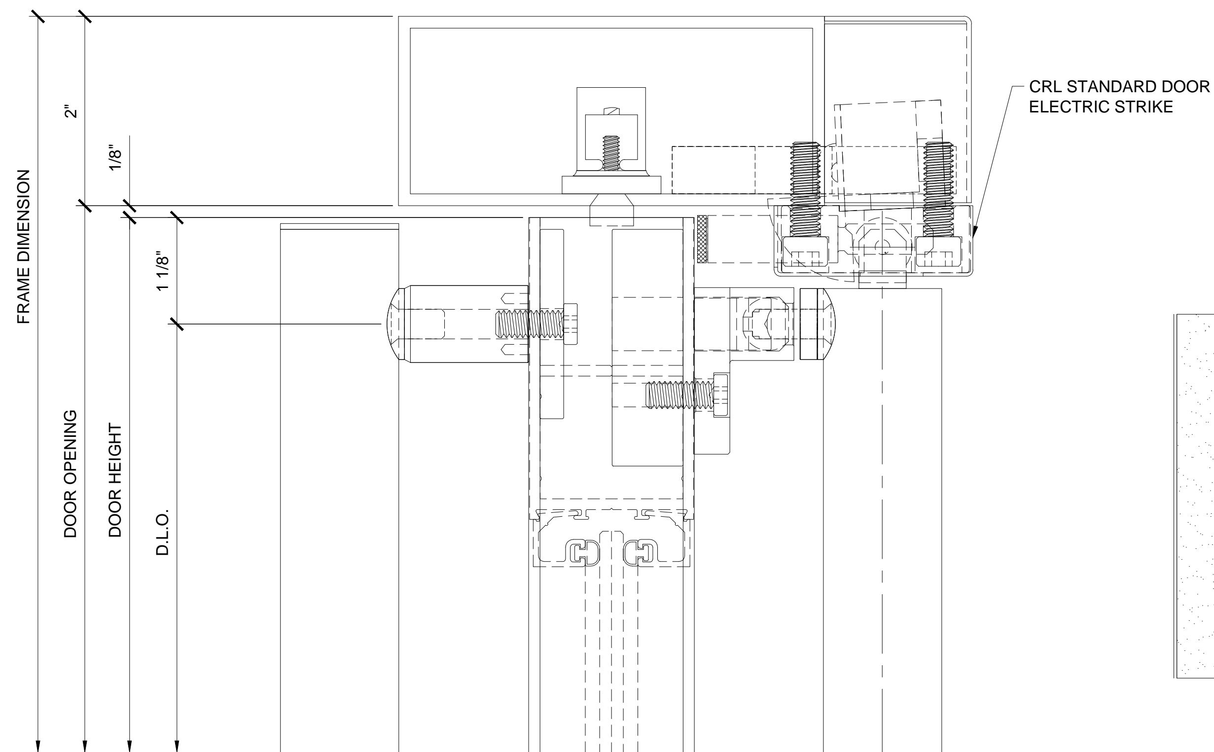
4 PANIC HANDLE DOOR HEAD DETAIL CRL-US ALUM SERIES 400 FULL FRAMED DOOR W/PA100F
