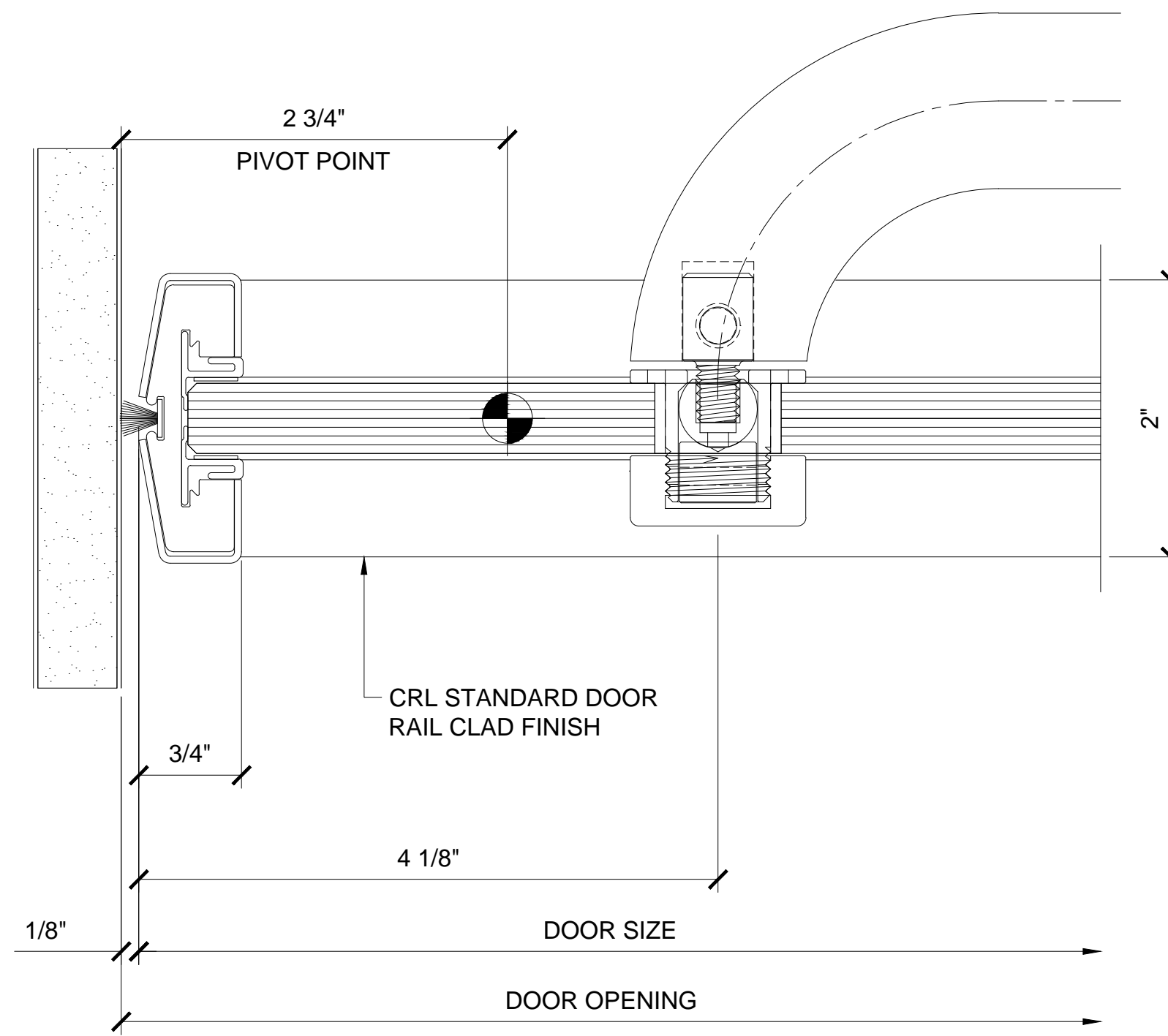
5 JAMB DETAIL AT PANIC HANDLE HINGE SIDE WEDGE-LOCK "P" STYLE ALL GLASS DOOR W/ PA100F
