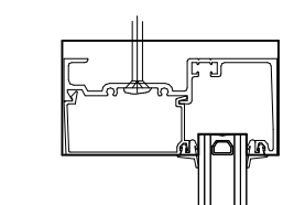
9 STOREFRONT FF451 @ HEADER 3" = 1'-0"
