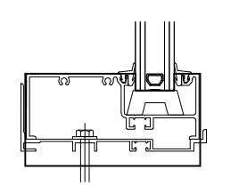
12 STOREFRONT FF451 @ SILL 3" = 1'-0"
