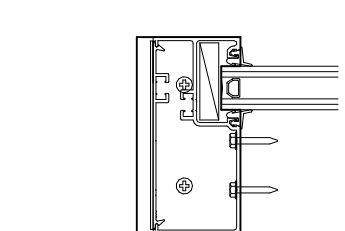
10 STOREFRONT FF451 @ JAMB 3" = 1'-0"
