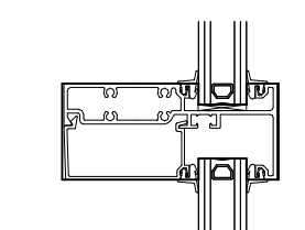
11 STOREFRONT FF451 @ RAIL 3" = 1'-0"
