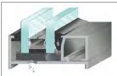
Cross Section of Tape Showing Shim
